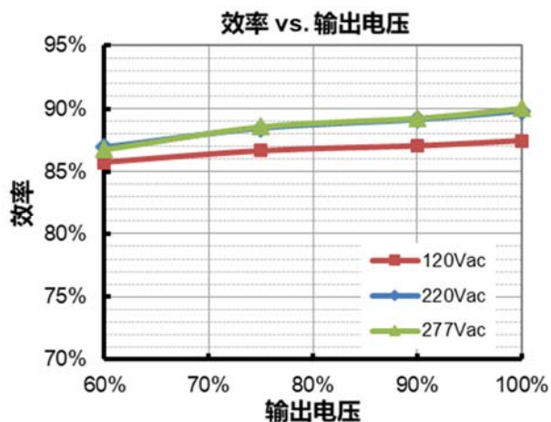
EUM-075S150SV( I_o=1500mA )
