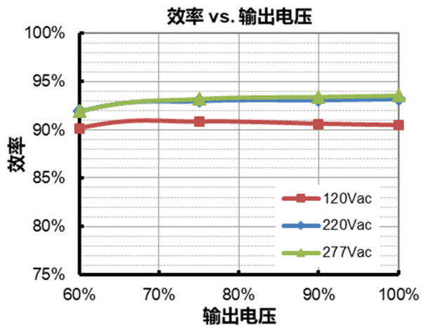
EUM-240S350SV( I_o=2150mA )
