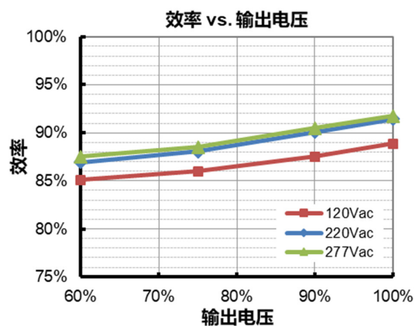
EUM-240S670SV( I_o=6700mA )
