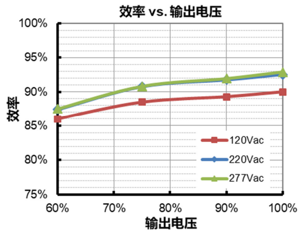
EUM-240S350SV( I_o=3500mA )
