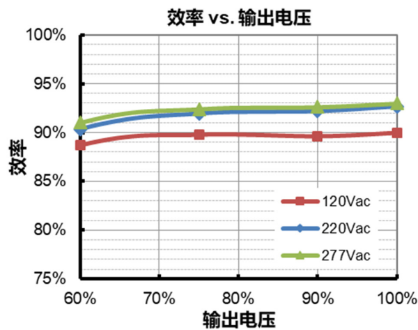
EUM-240S670SV( I_o=4200mA )
