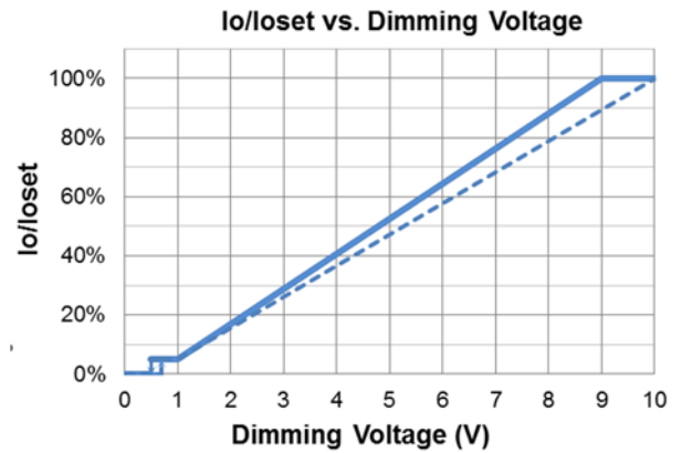
Implementation 1: Positive logic
