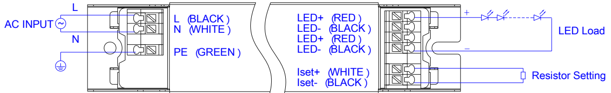
Wire Connection 1
